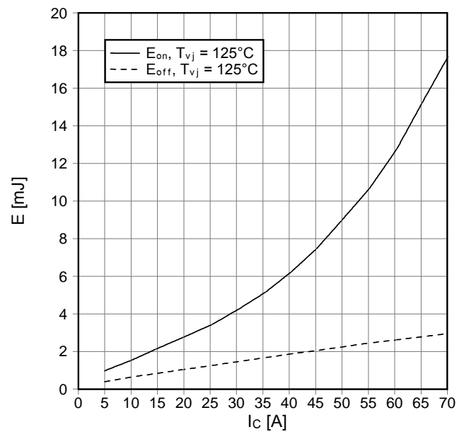
Schaltverluste IGBT-Wechselr. (typisch) switching losses IGBT-inverter (typical) E_{on} = f(I_C), E_{off} = f(I_C) V_{GE} = \pm 15\text{ V}, R_{Gon} = 30\ \Omega, R_{Goff} = 30\ \Omega, V_{CE} = 600\text{ V}
